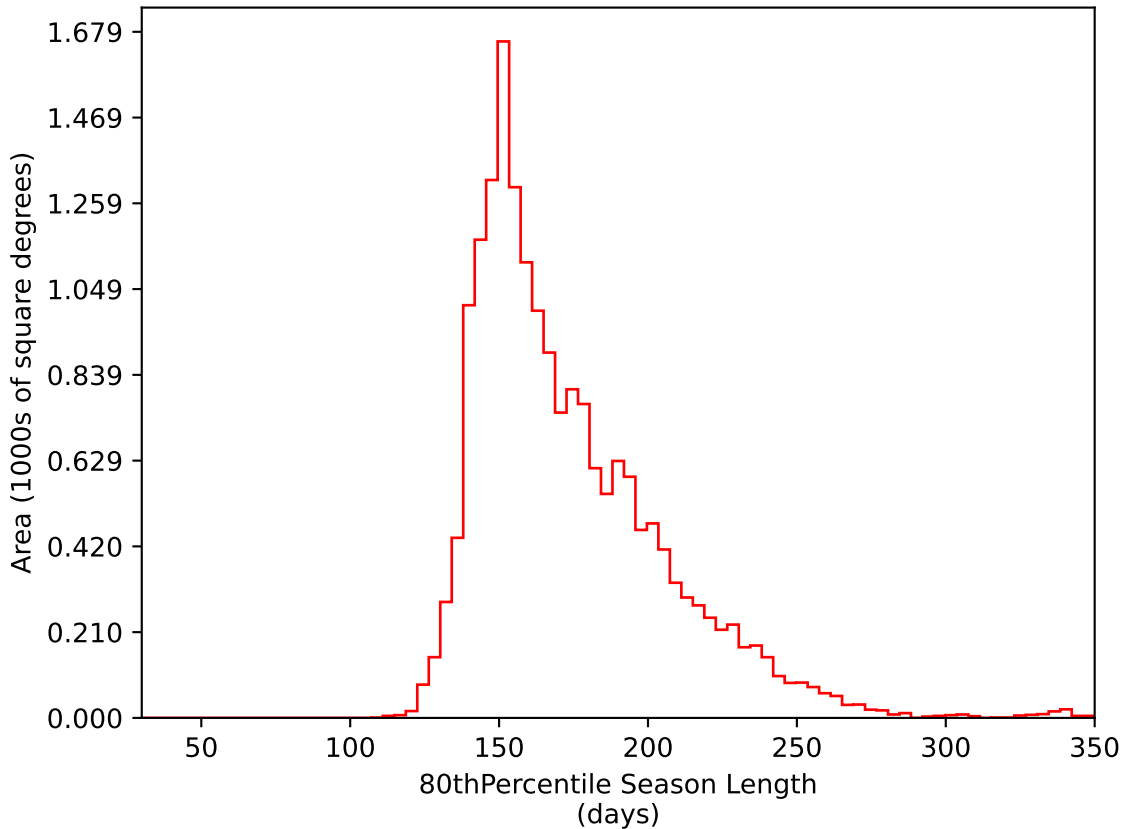
weather_cloudso35v3.4_10yrs WFD i band: 80thPercentile Season Length
