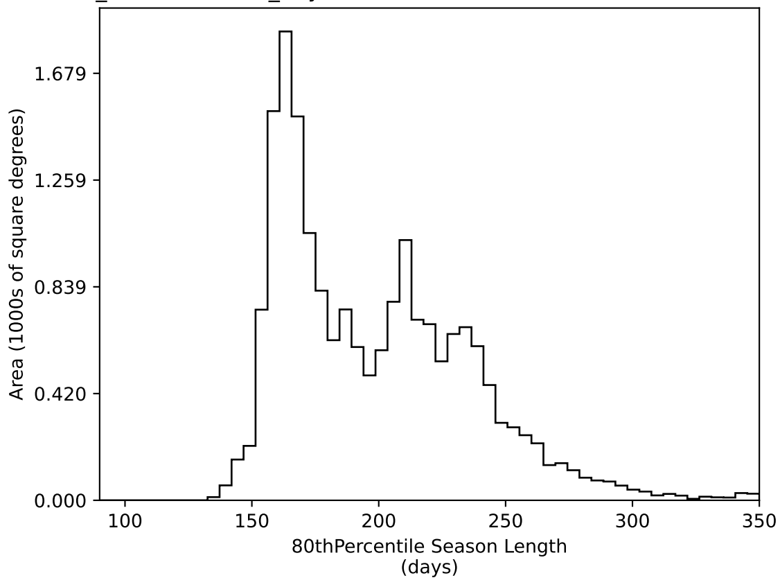
weather_cloudso35v3.4_10yrs WFD all bands: 80thPercentile Season Length
