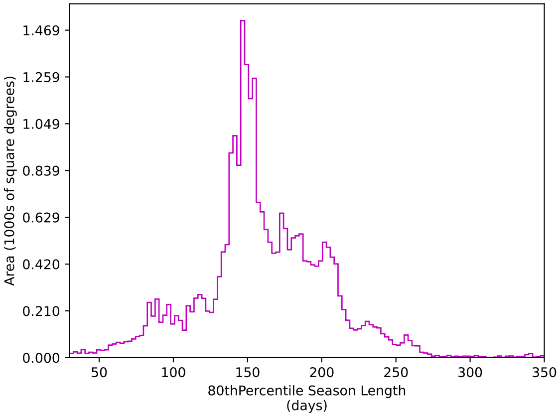
weather_cloudso35v3.4_10yrs All sky z band: 80thPercentile Season Length
