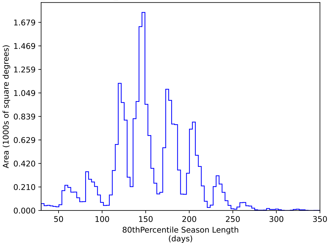
weather_cloudso35v3.4_10yrs All sky y band: 80thPercentile Season Length
