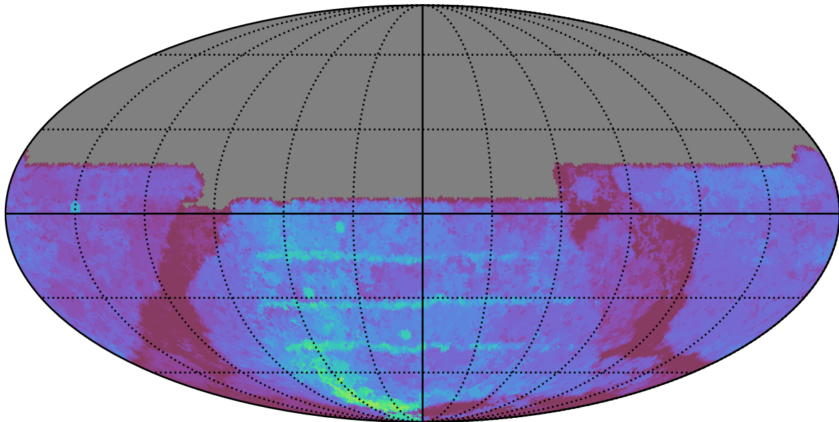
weather_cloudso35v3.4_10yrs All sky u band: 80thPercentile Season Length
