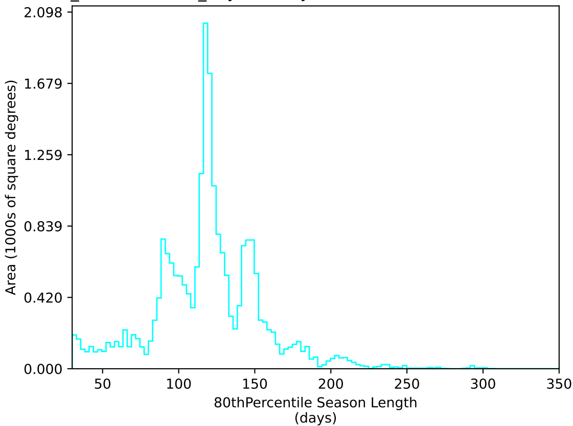
weather_cloudso35v3.4_10yrs All sky u band: 80thPercentile Season Length
