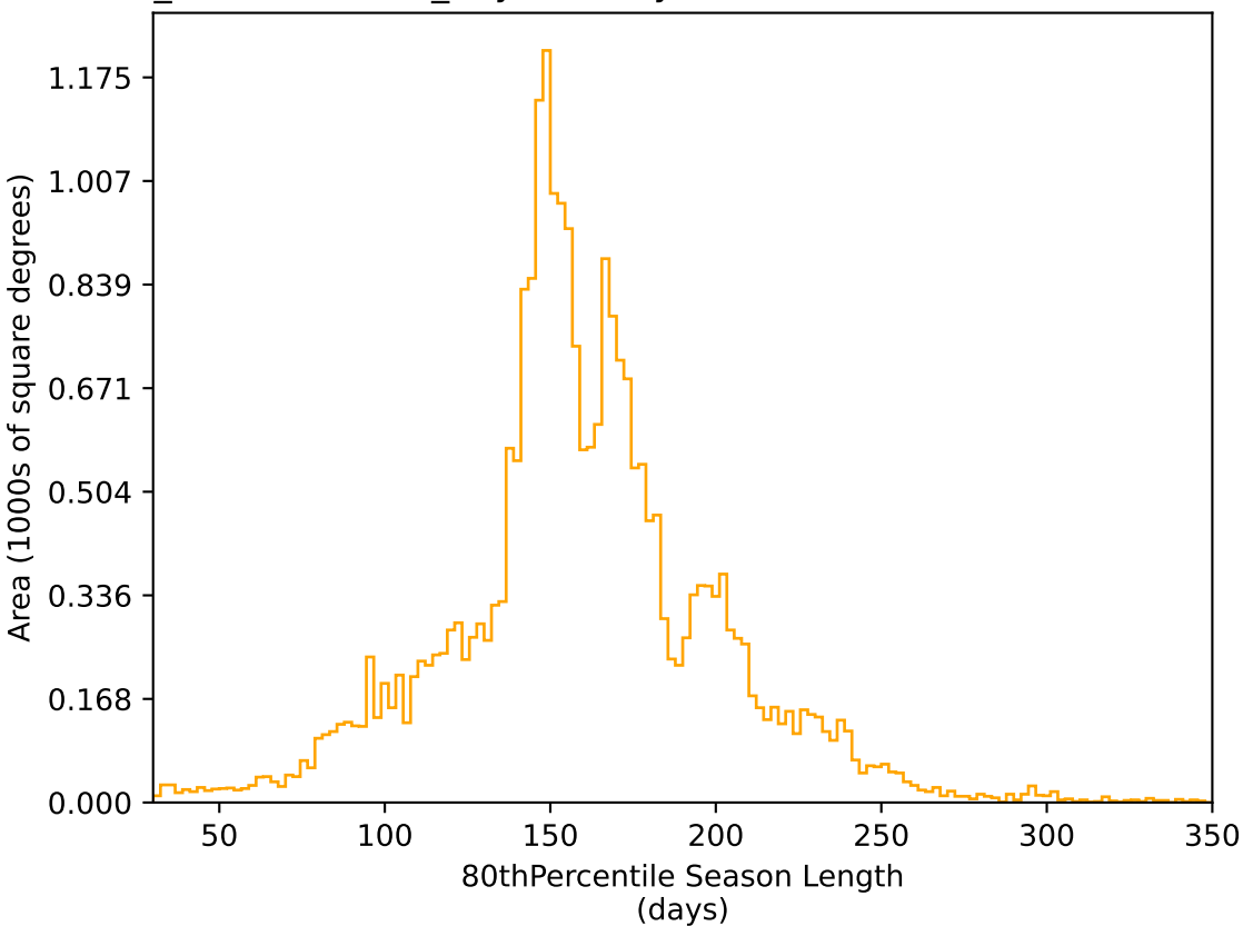
weather_cloudso35v3.4_10yrs All sky r band: 80thPercentile Season Length
