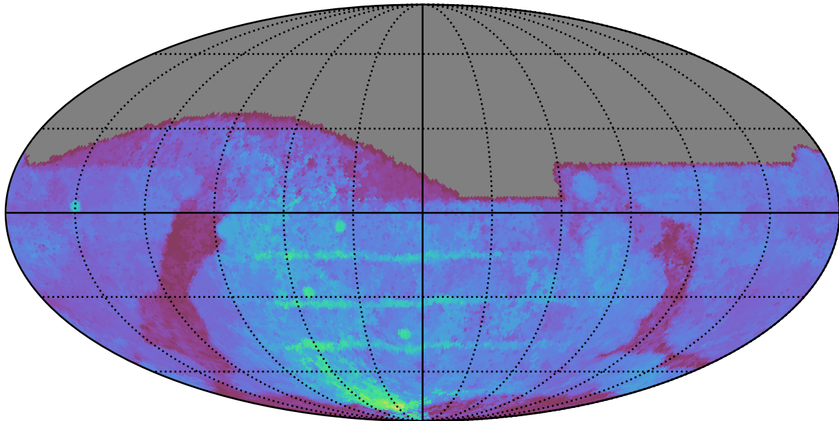
weather_cloudso35v3.4_10yrs All sky g band: 80thPercentile Season Length
