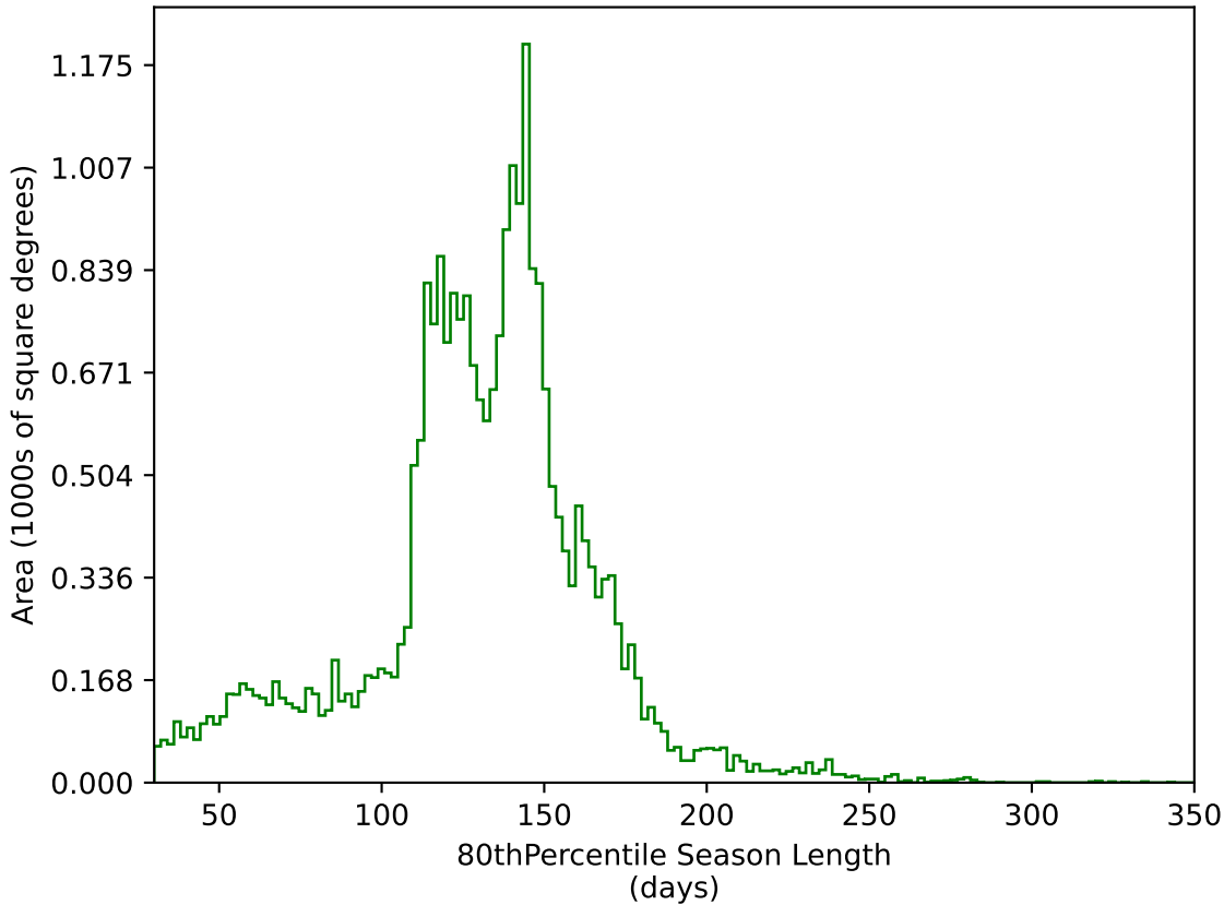
weather_cloudso35v3.4_10yrs All sky g band: 80thPercentile Season Length
