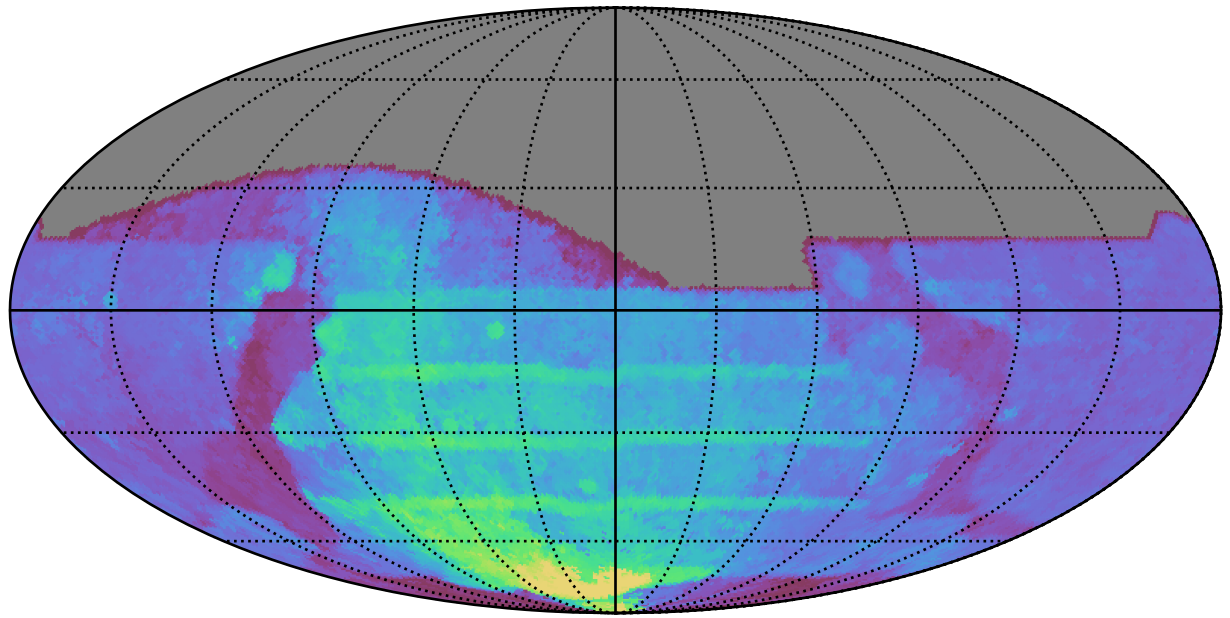
weather_cloudso35v3.4_10yrs All sky all bands: 80thPercentile Season Length
