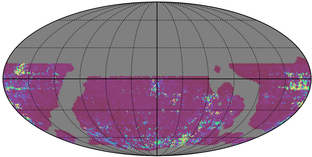
weather_cloudso35v3.4_10yrs WFD z band: 75th Percentile Intranight Timespan
