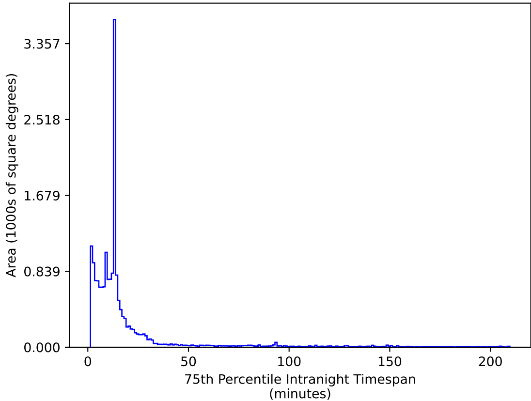
weather_cloudso35v3.4_10yrs WFD z band: 75th Percentile Intranight Timespan
