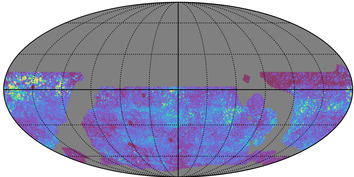
weather_cloudso35v3.4_10yrs WFD y band: 75th Percentile Intranight Timespan
