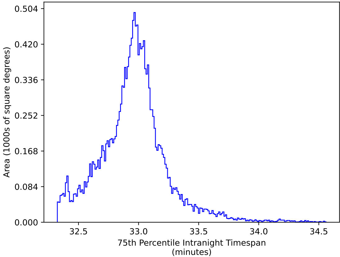
weather_cloudso35v3.4_10yrs WFD y band: 75th Percentile Intranight Timespan
