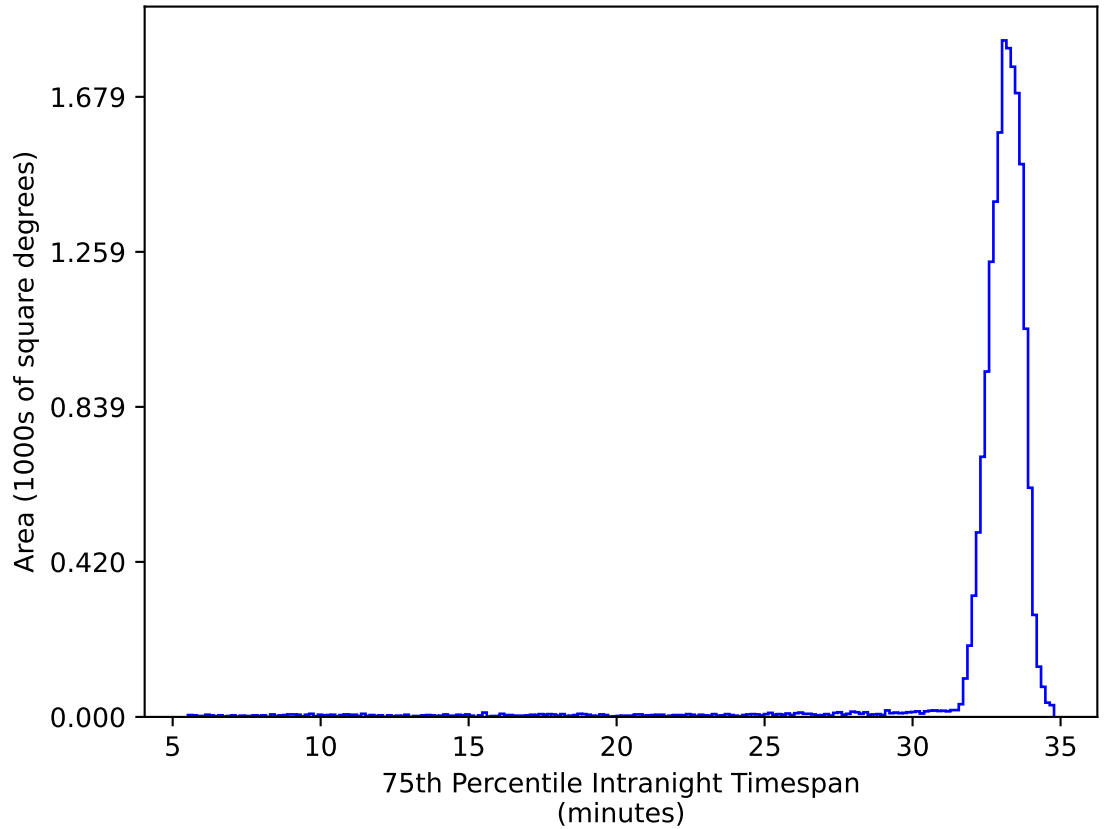
weather_cloudso35v3.4_10yrs WFD ug bands: 75th Percentile Intranight Timespan
