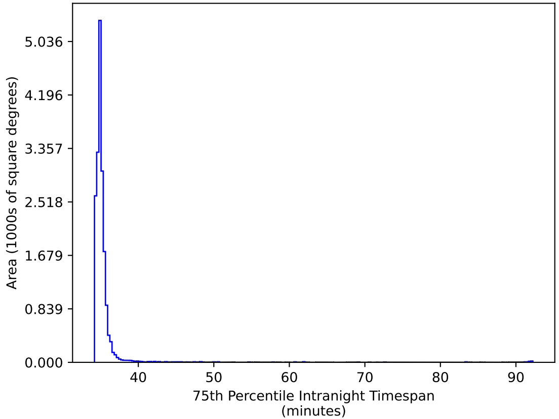
weather_cloudso35v3.4_10yrs WFD ri bands: 75th Percentile Intranight Timespan
