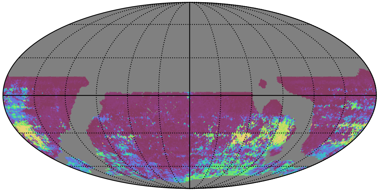
weather_cloudso35v3.4_10yrs WFD r band: 75th Percentile Intranight Timespan
