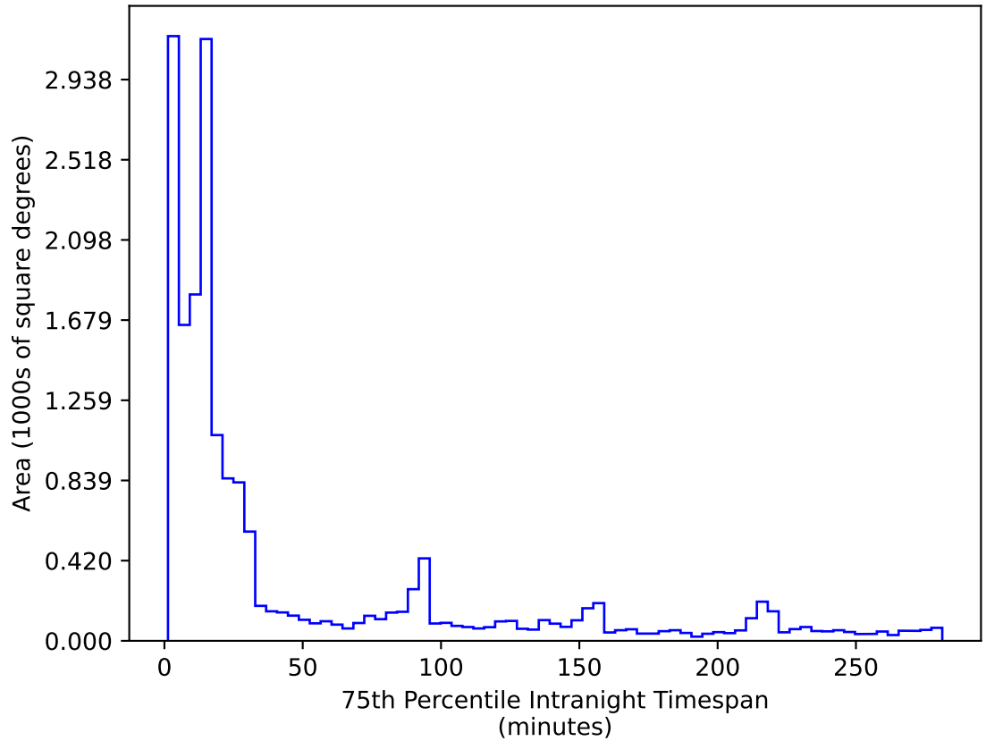
weather_cloudso35v3.4_10yrs WFD r band: 75th Percentile Intranight Timespan
