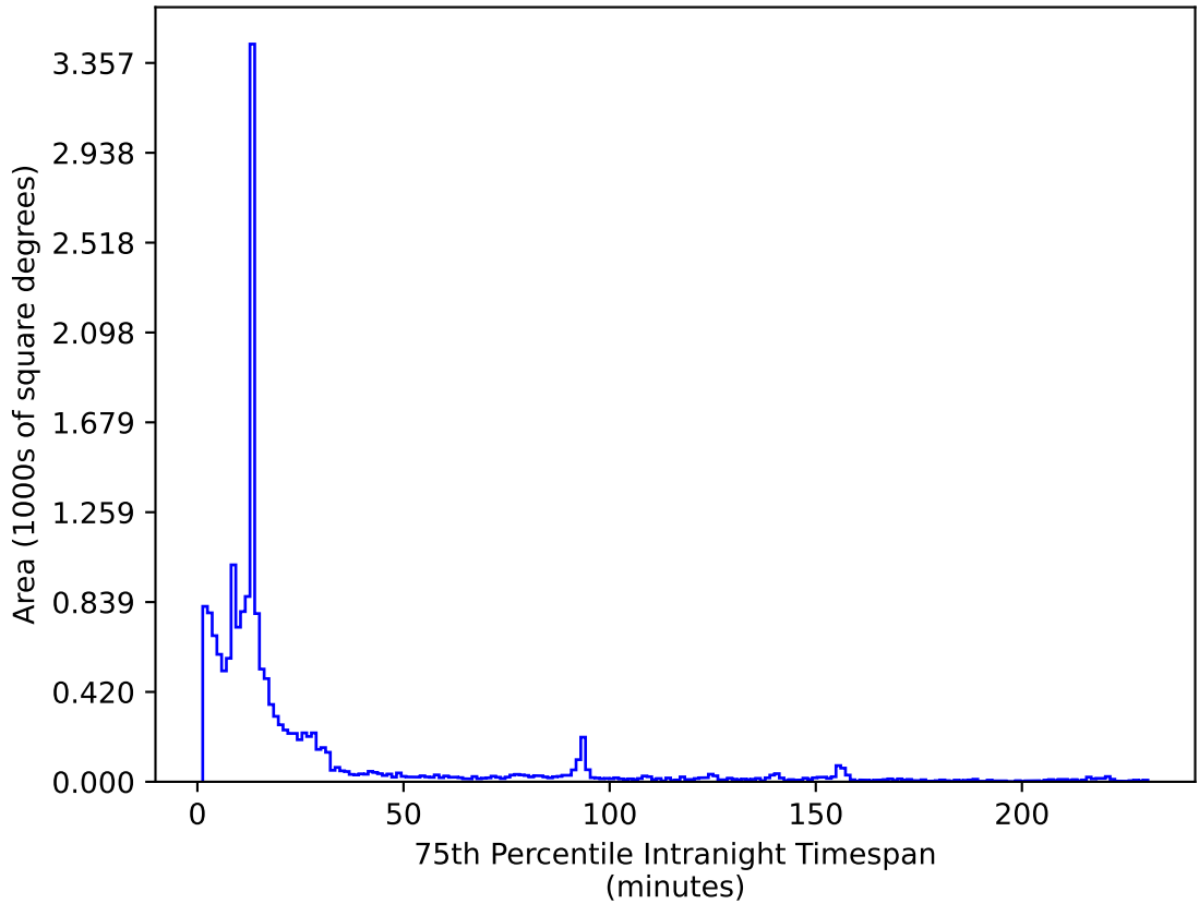
weather_cloudso35v3.4_10yrs WFD i band: 75th Percentile Intranight Timespan
