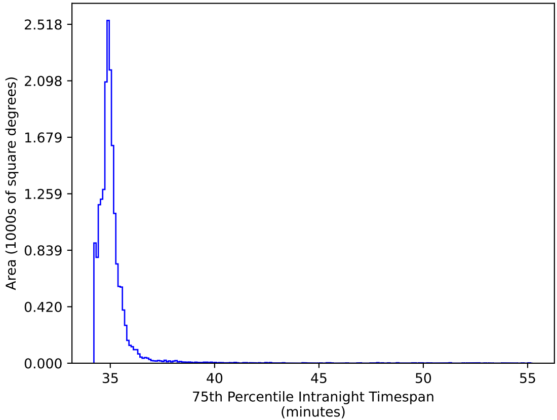
weather_cloudso35v3.4_10yrs WFD gr bands: 75th Percentile Intranight Timespan
