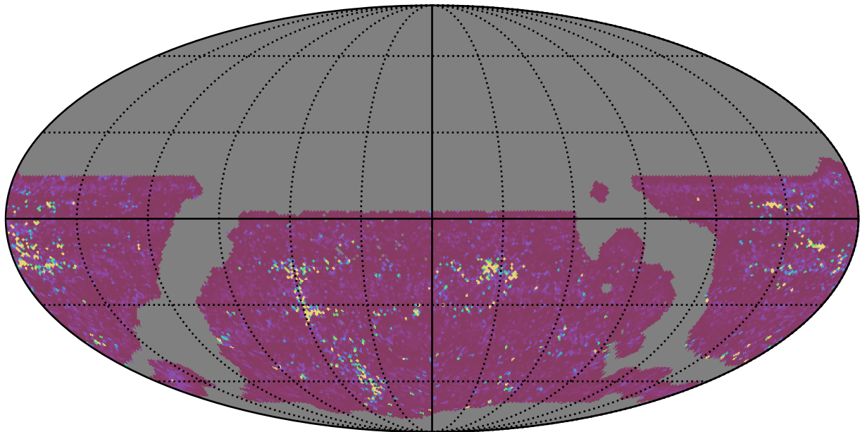
weather_cloudso35v3.4_10yrs WFD g band: 75th Percentile Intranight Timespan
