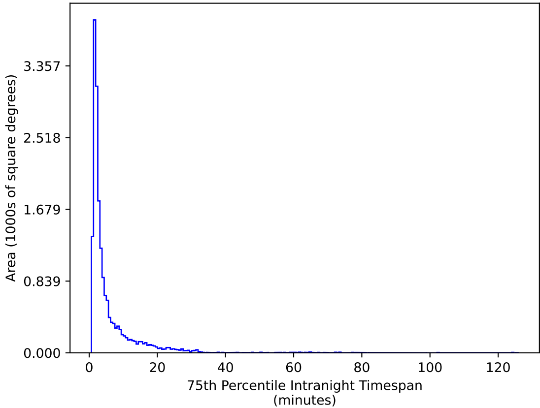
weather_cloudso35v3.4_10yrs WFD g band: 75th Percentile Intranight Timespan
