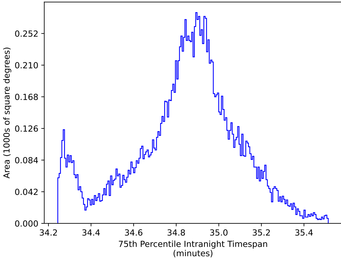
weather_cloudso35v3.4_10yrs WFD: 75th Percentile Intranight Timespan
