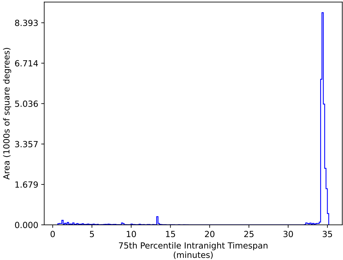
weather_cloudso35v3.4_10yrs All sky zy bands: 75th Percentile Intranight Timespan
