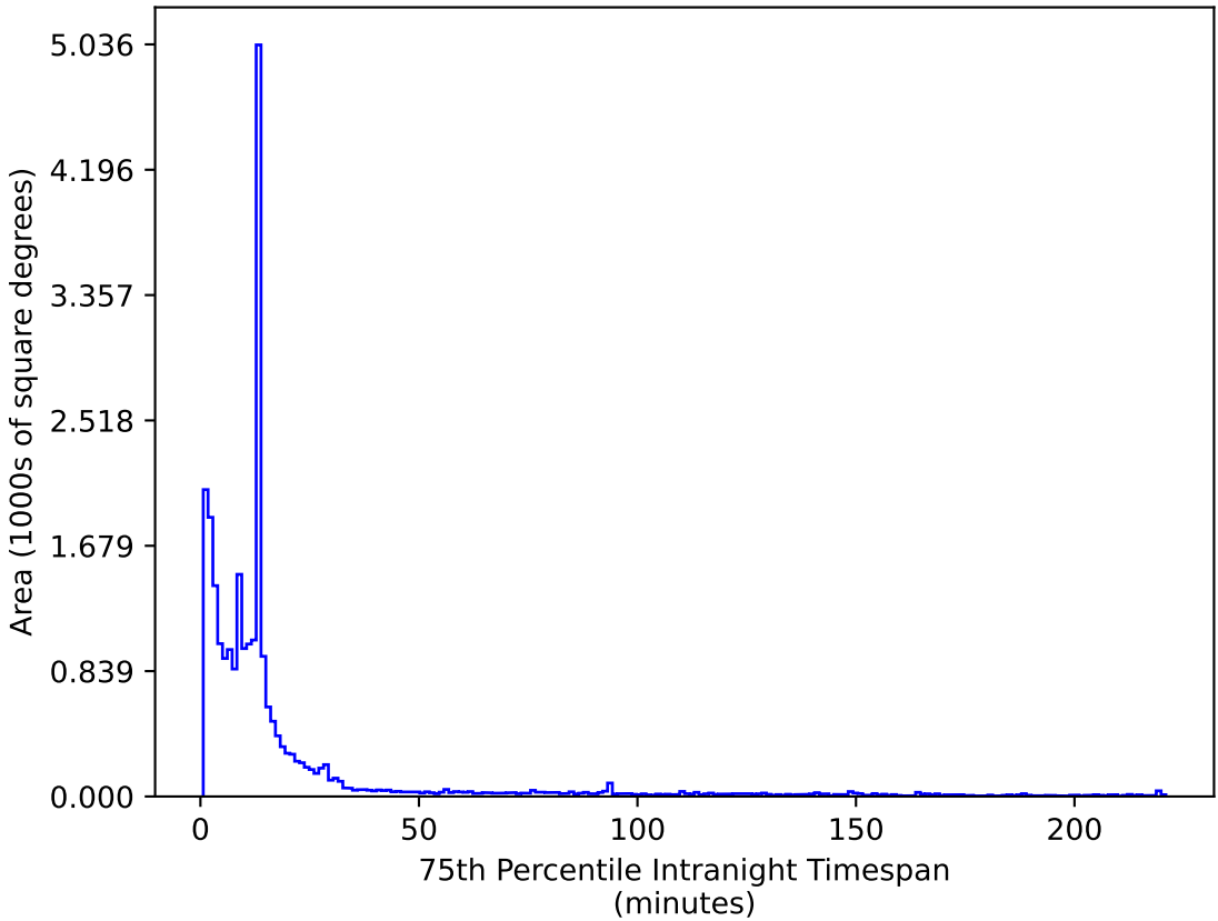
weather_cloudso35v3.4_10yrs All sky z band: 75th Percentile Intranight Timespan
