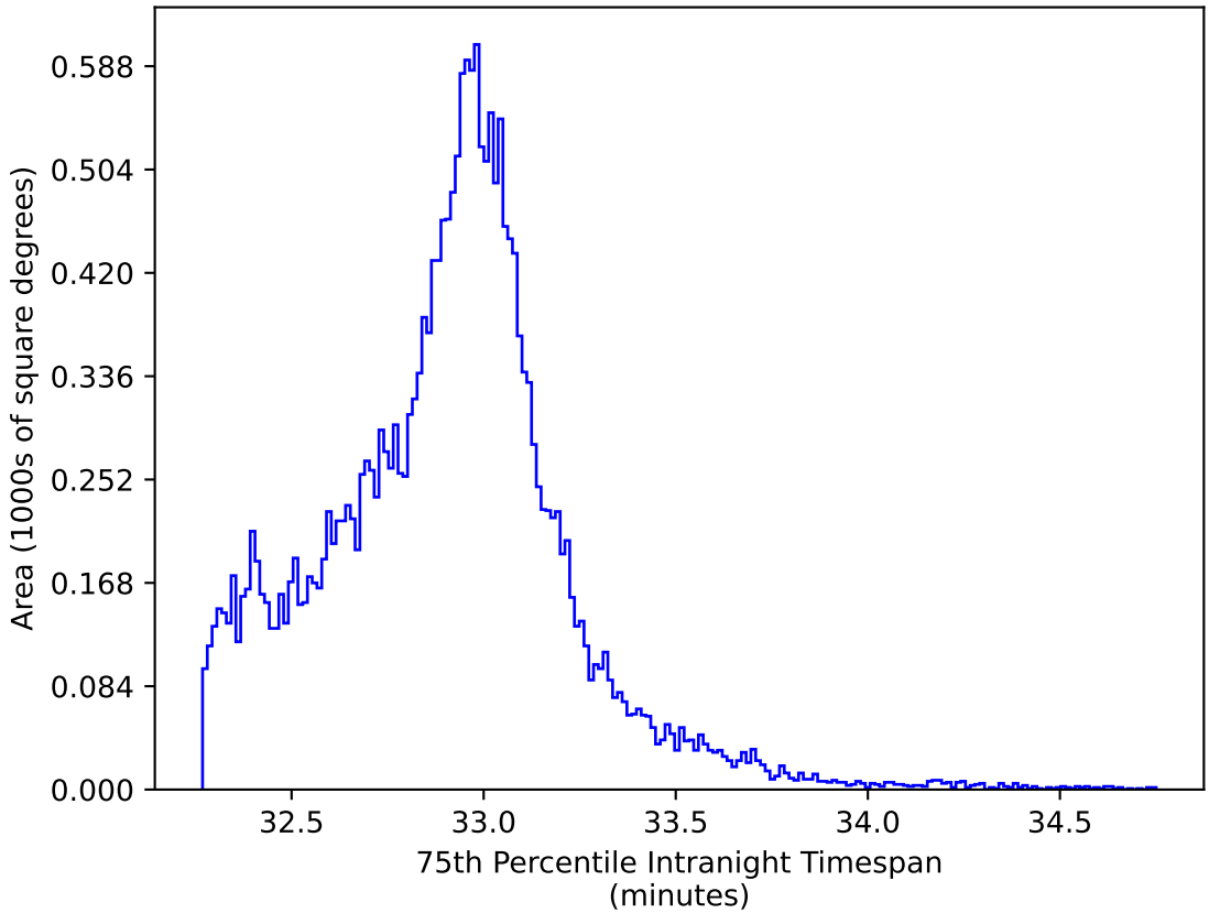
weather_cloudso35v3.4_10yrs All sky y band: 75th Percentile Intranight Timespan
