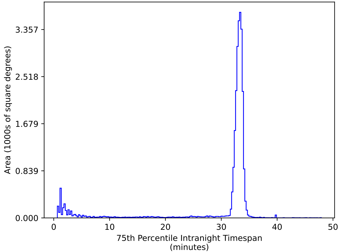
weather_cloudso35v3.4_10yrs All sky ug bands: 75th Percentile Intranight Timespan
