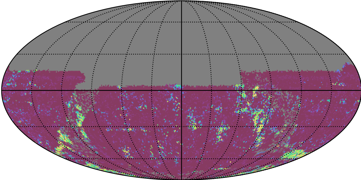
weather_cloudso35v3.4_10yrs All sky u band: 75th Percentile Intranight Timespan
