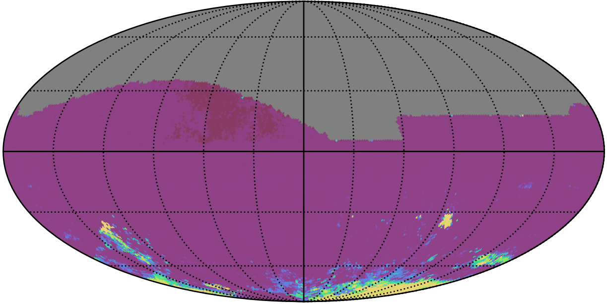
weather_cloudso35v3.4_10yrs All sky ri bands: 75th Percentile Intranight Timespan
