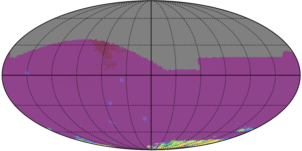
weather_cloudso35v3.4_10yrs All sky iz bands: 75th Percentile Intranight Timespan
