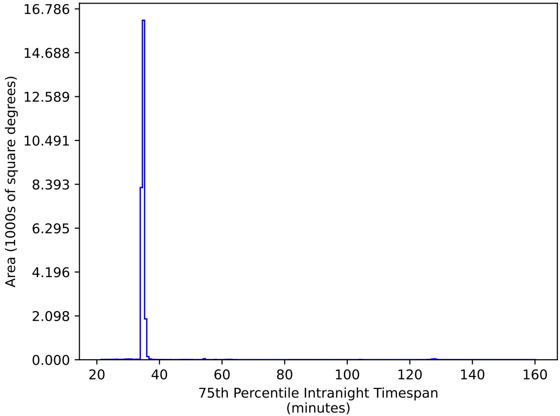
weather_cloudso35v3.4_10yrs All sky iz bands: 75th Percentile Intranight Timespan
