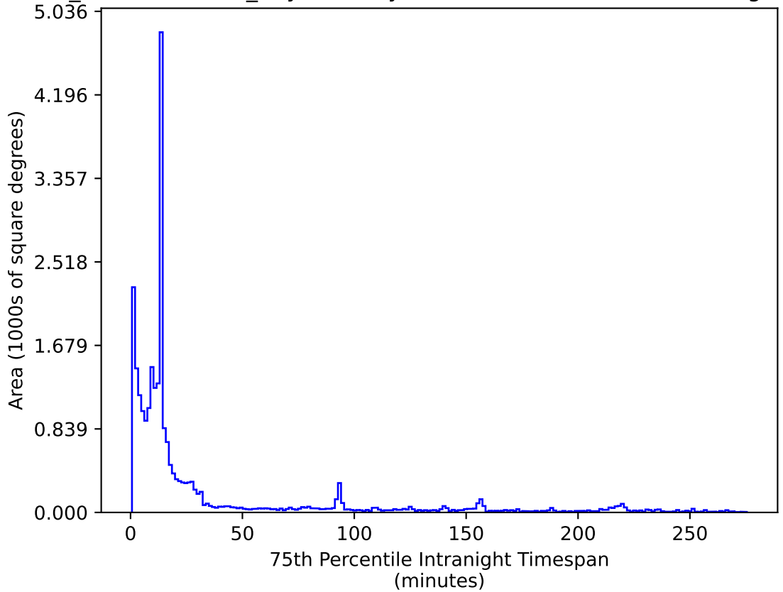
weather_cloudso35v3.4_10yrs All sky i band: 75th Percentile Intranight Timespan
