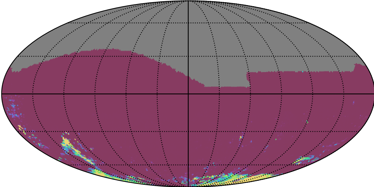
weather_cloudso35v3.4_10yrs All sky gr bands: 75th Percentile Intranight Timespan
