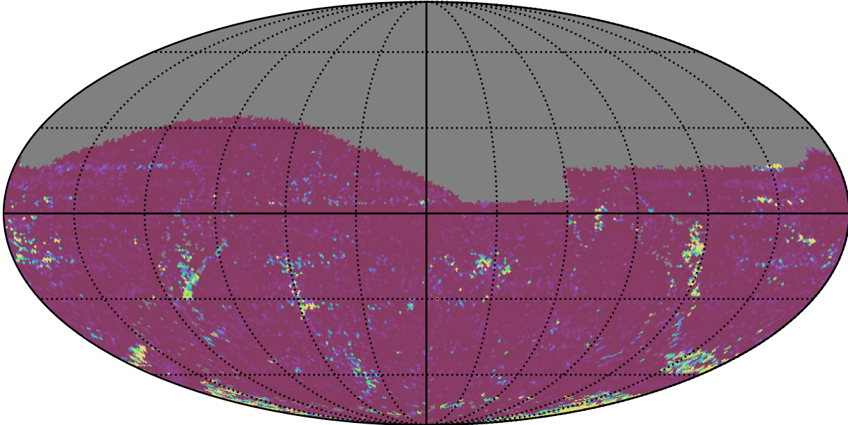
weather_cloudso35v3.4_10yrs All sky g band: 75th Percentile Intranight Timespan
