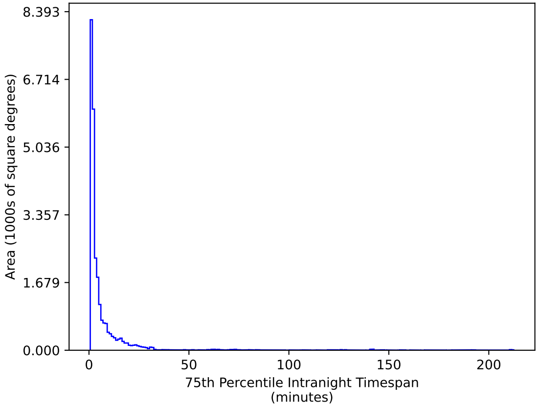
weather_cloudso35v3.4_10yrs All sky g band: 75th Percentile Intranight Timespan
