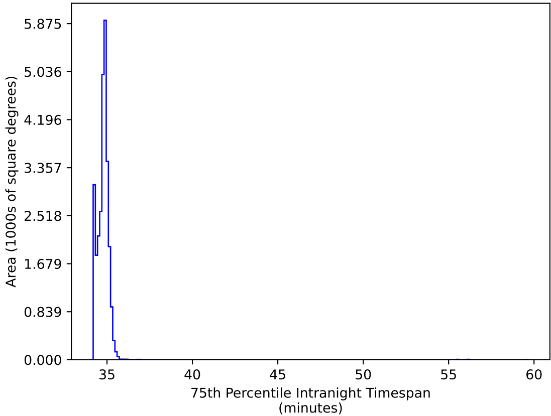
weather_cloudso35v3.4_10yrs All sky all bands: 75th Percentile Intranight Timespan
