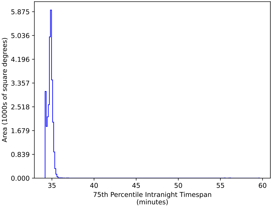
weather_cloudso35v3.4_10yrs All sky: 75th Percentile Intranight Timespan
