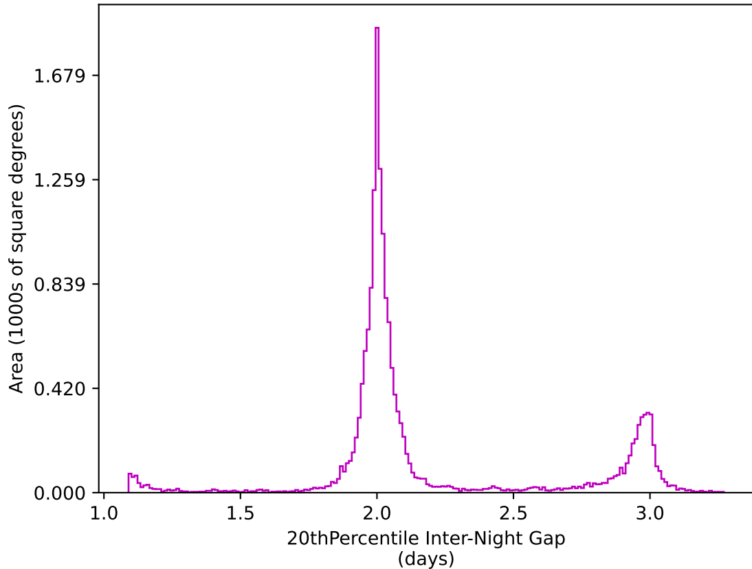
weather_cloudso35v3.4_10yrs WFD z band: 20thPercentile Inter-Night Gap
