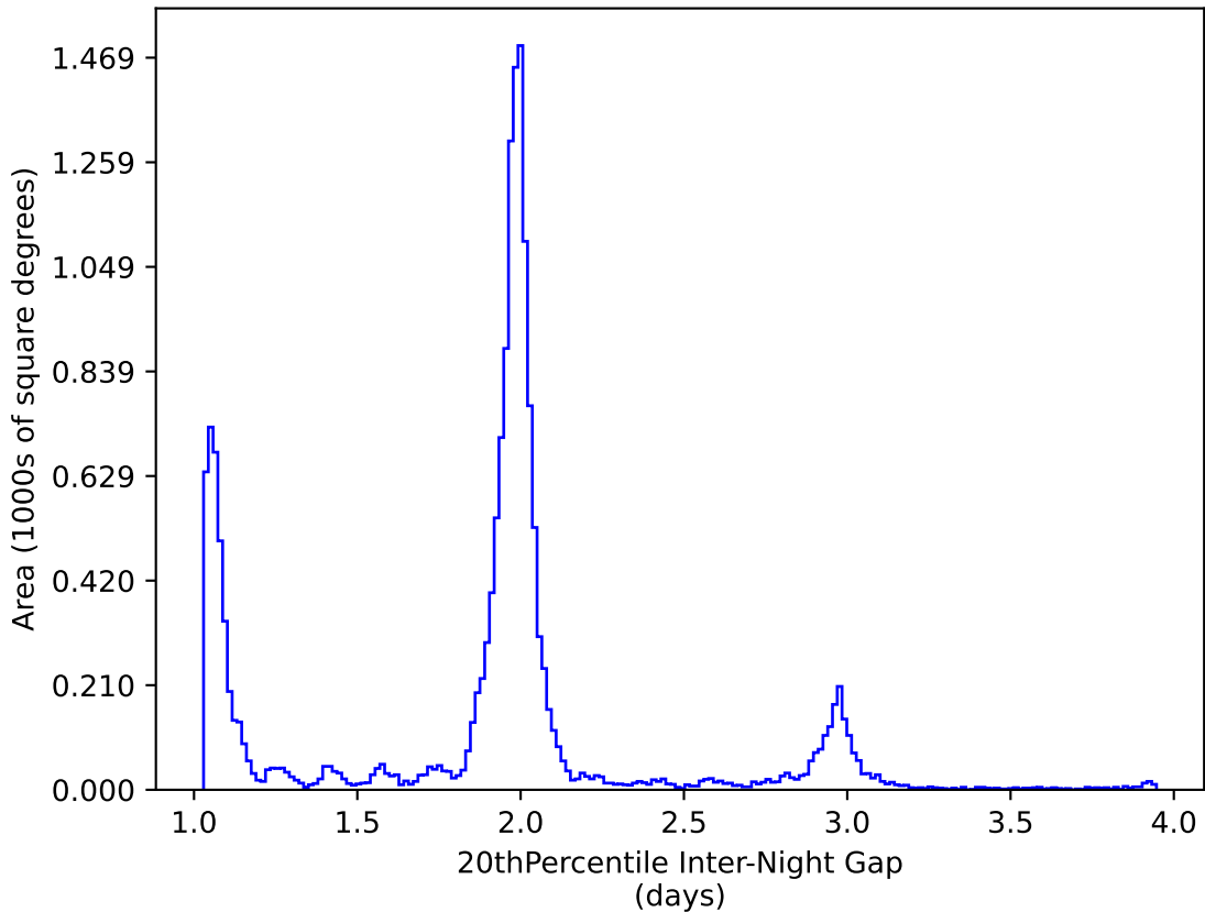
weather_cloudso35v3.4_10yrs WFD y band: 20thPercentile Inter-Night Gap
