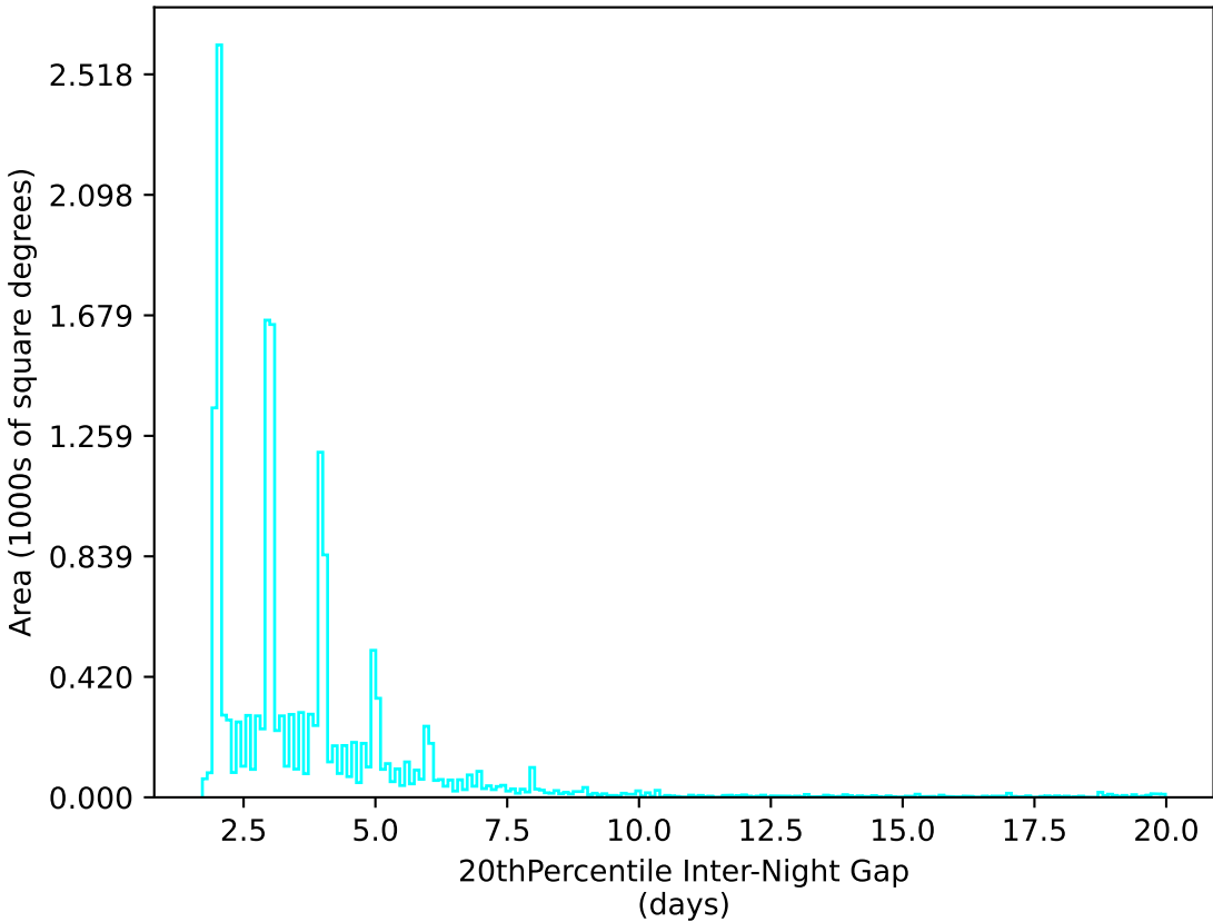
weather_cloudso35v3.4_10yrs WFD u band: 20thPercentile Inter-Night Gap
