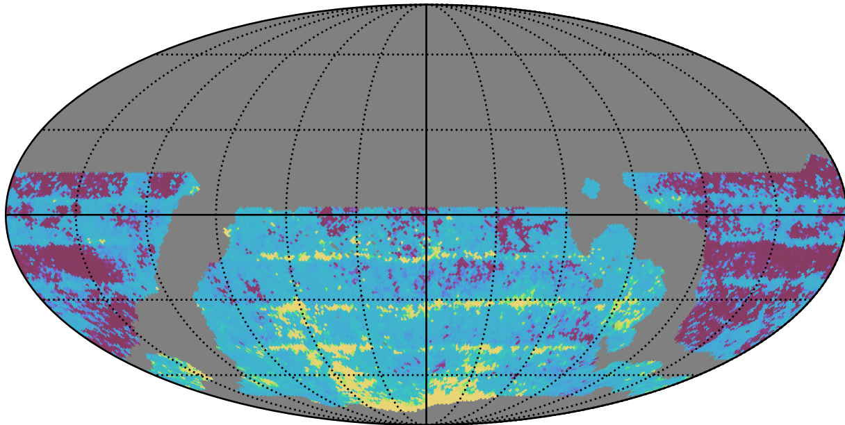
weather_cloudso35v3.4_10yrs WFD r band: 20thPercentile Inter-Night Gap
