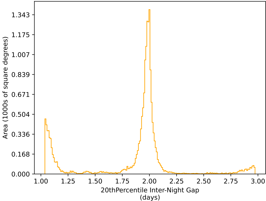
weather_cloudso35v3.4_10yrs WFD r band: 20thPercentile Inter-Night Gap
