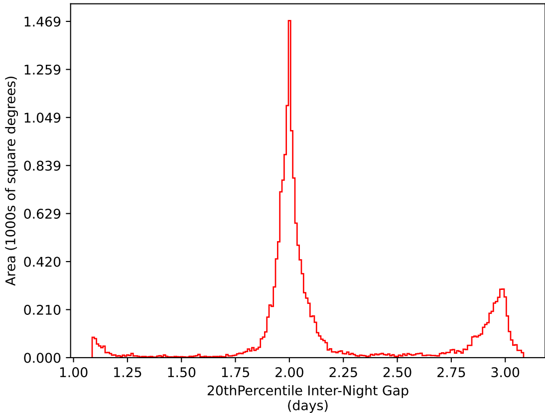
weather_cloudso35v3.4_10yrs WFD i band: 20thPercentile Inter-Night Gap
