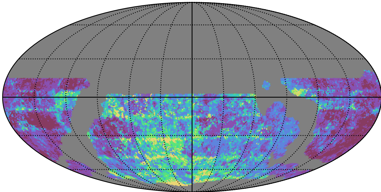
weather_cloudso35v3.4_10yrs WFD g band: 20thPercentile Inter-Night Gap
