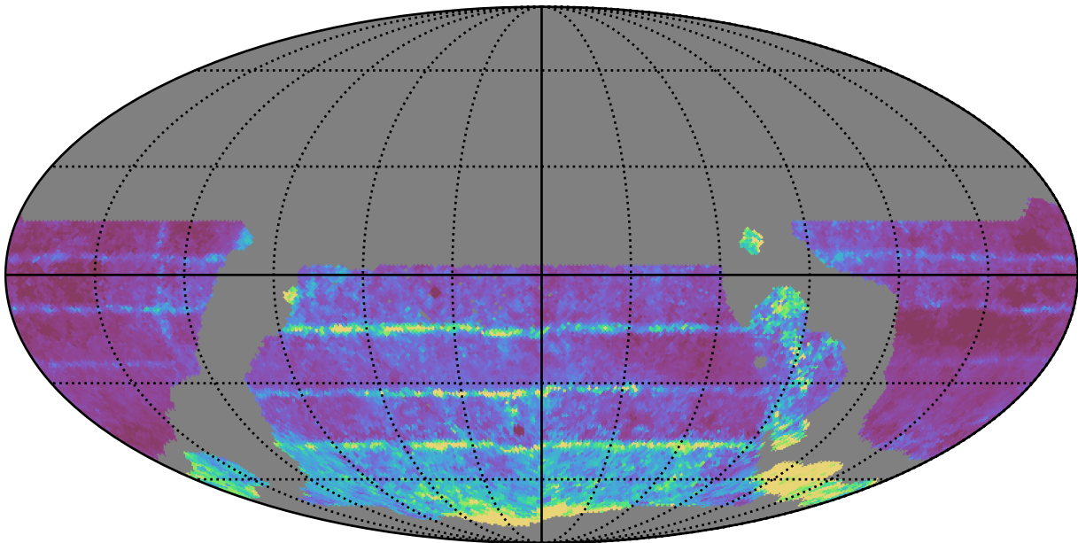
weather_cloudso35v3.4_10yrs WFD all bands: 20thPercentile Inter-Night Gap
