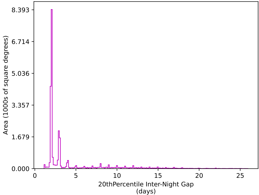
weather_cloudso35v3.4_10yrs All sky z band: 20thPercentile Inter-Night Gap
