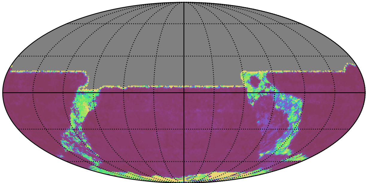
weather_cloudso35v3.4_10yrs All sky y band: 20thPercentile Inter-Night Gap
