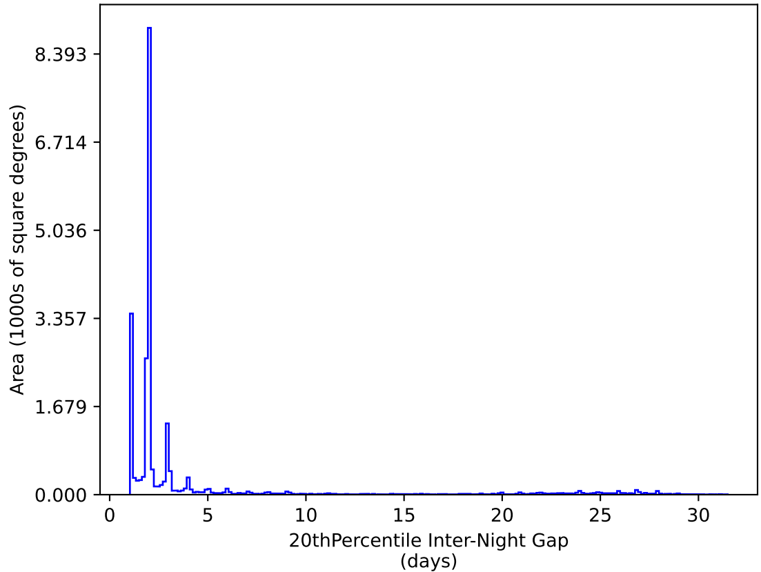
weather_cloudso35v3.4_10yrs All sky y band: 20thPercentile Inter-Night Gap
