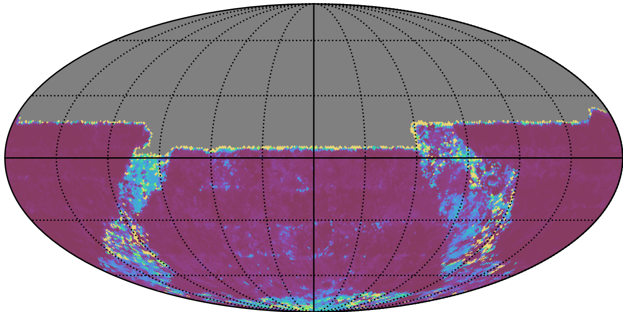
weather_cloudso35v3.4_10yrs All sky u band: 20thPercentile Inter-Night Gap
