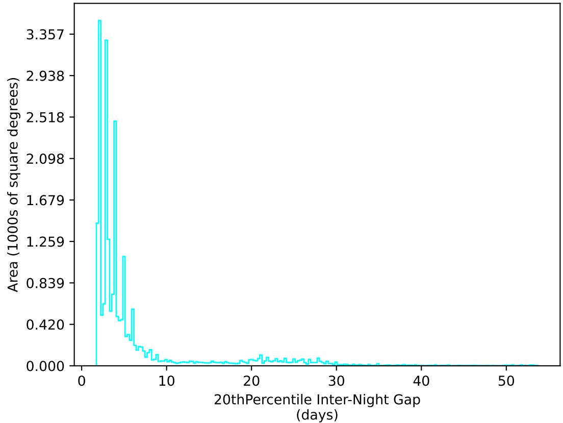
weather_cloudso35v3.4_10yrs All sky u band: 20thPercentile Inter-Night Gap
